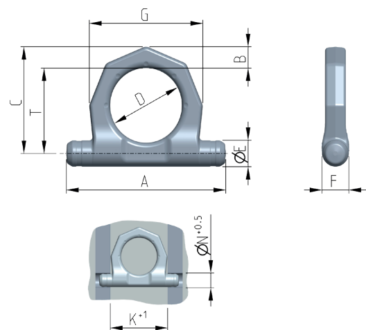
Pic. 4: Dimensioning Lashing Ring (integrated in the design)
