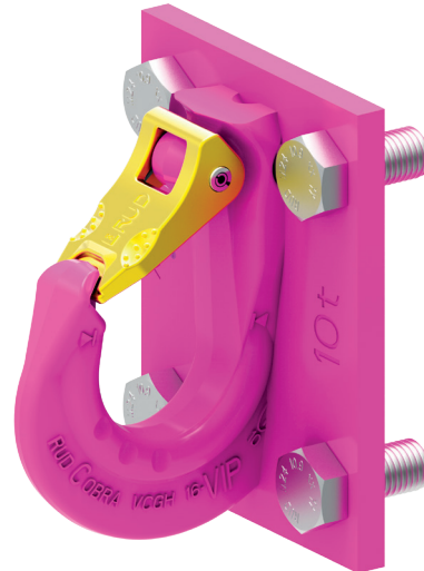
Excavator hook for bolting VCGH-G
