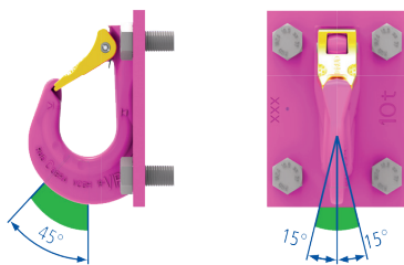
Pic. 1: Permissible load direction
